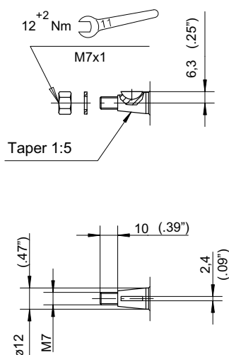
Shaft end
