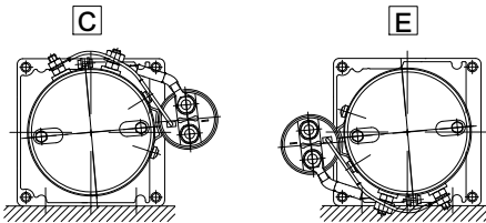
Relay mounting positions Standard positions
