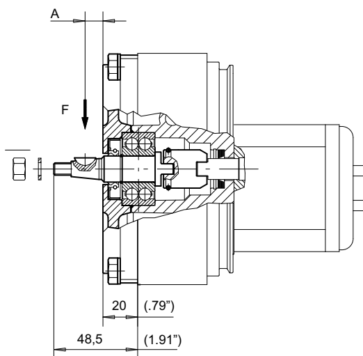
Shaft end
