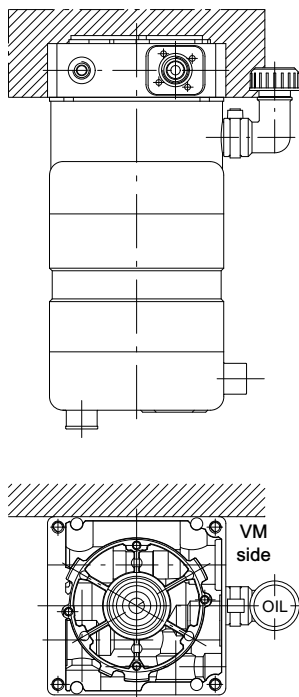
Assembling position P45
