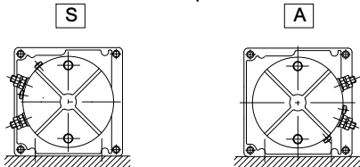
Standard positions
