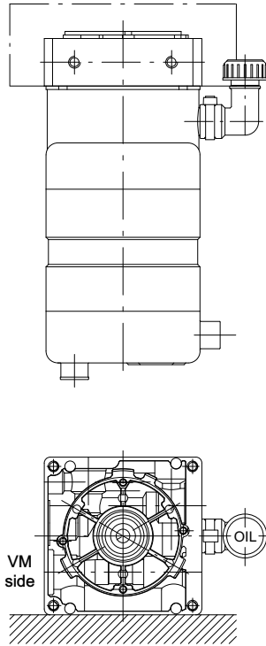
Assembling position P35
