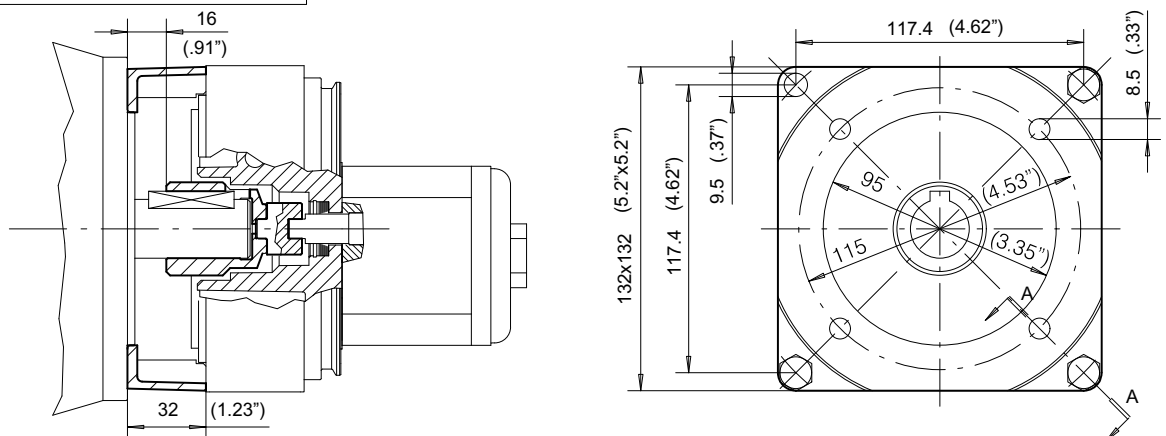
(A) Motor coupling: 200659400230
