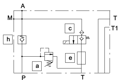
Same example without flow control
