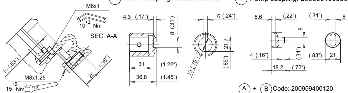
(A) Motor coupling 200659400190
