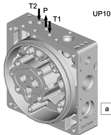
T2 P T1
