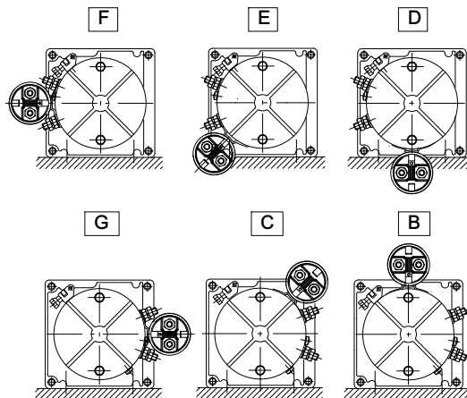
Relay mounting positions
