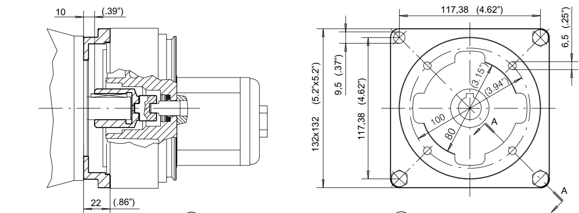
(A) Motor coupling 200659400190
