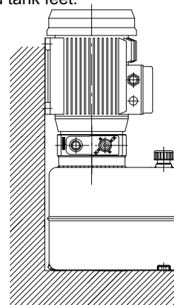
Vertical assembling for power pack with plastic/metal tanks
