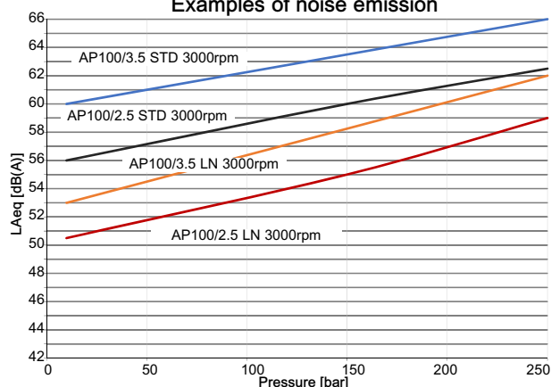
Low Noise versions Vs standard gears Examples of noise emission
