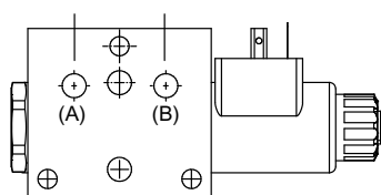
Valve with one solenoid "B" - Circuit: C-01
