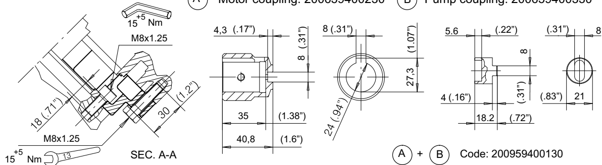
(A) Motor coupling: 200659400230
