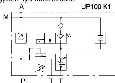
Typical hydraulic circuits
