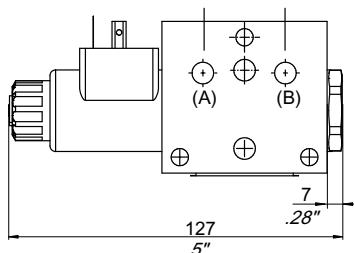
Valve with one solenoid "B" - Circuit: C-01
