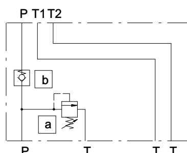
Example of standard circuit UP100K4D0-01
