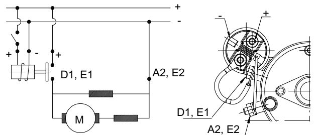
Electric diagram
